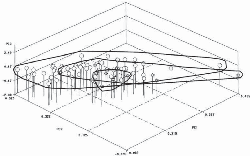
Fig. 2. Three-dimensional scatter plotting of OTUs representing I. excisus complex. Icons indicate pre-identification of OTUs before the PCA based on the morphological characters indicated in the original descriptions. Balloons, EXCISUS; cubes, COREANUS; stars, CHIISANENSIS.
